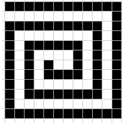
Figure 3.3: An object with \Theta(WH) pixels and with a diameter in \Theta(WH) . Example for the lower bound of \Omega(WH) for any centralized algorithm and for any distributed algorithm that stays within the object.
