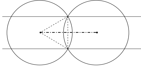
Figure 4.11: Two scan points with distance \sqrt{3} \cdot r to each other: The dashed lines indicate a length of r , so, the dash-dotted line has a length of \sqrt{3} \cdot r , the distance of two scans.
