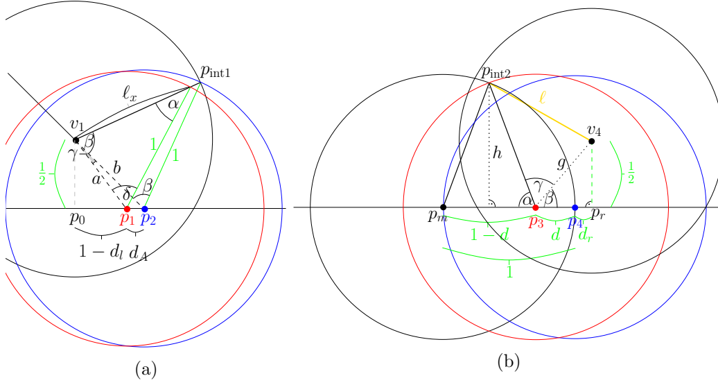
Figure 5.10: (a) \ell_x < 1 . (b) \ell < 1 .
