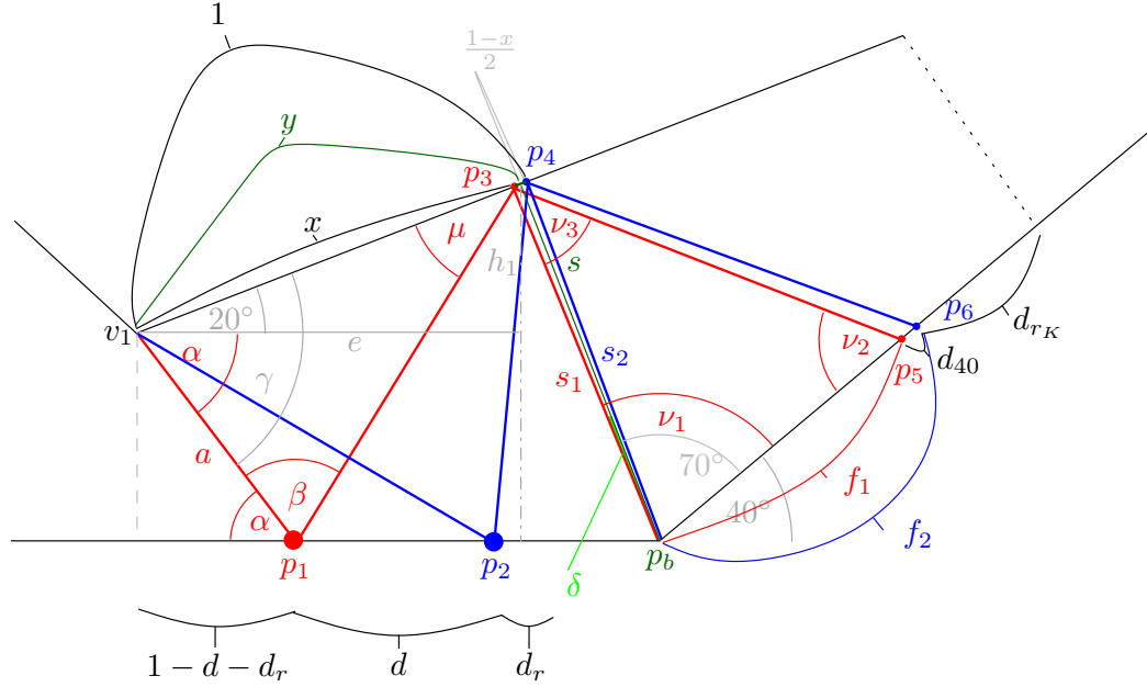
Figure 5.13: Construction of a 40°-bend of a corridor.
