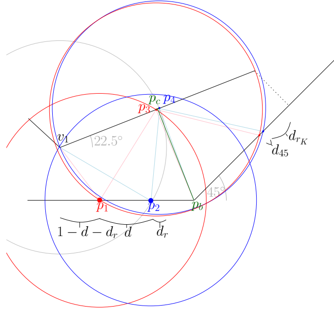
Figure 5.11: Construction of a 45°-bend of a corridor.
